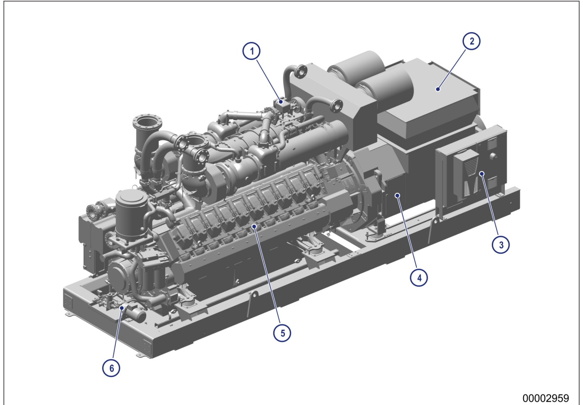
Figure 3: Engine-generator set – 20V engine, engine side
